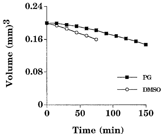
FIG. 3. Volume changes in zebrafish embryo as a function of time in 2 M DMSO ( n = 7 ) and 2 M PG ( n = 9 ) at 22\text{--}23^\circ\text{C} measured with light microscopy. A decrease of approximately 20% in the averaged volume was observed. The data from each group were averaged and normalized to a standard volume of 0.2 \text{ mm}^3 for each graph.
